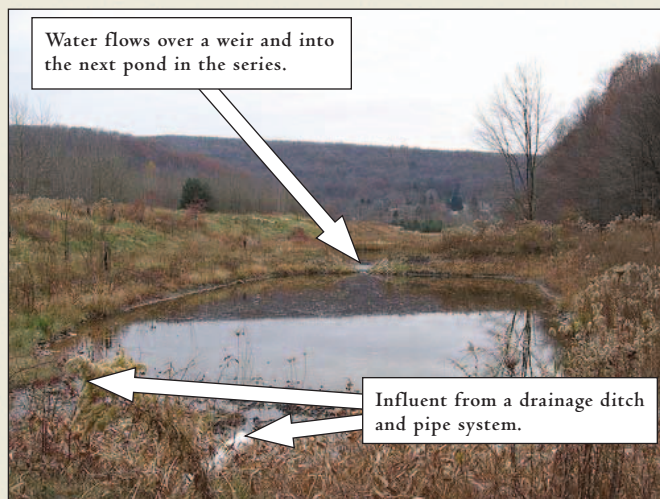
Figure 1. Simple settling pond system.
